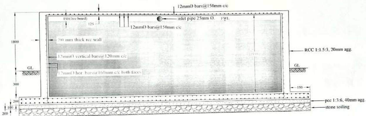
SECTION E-E
