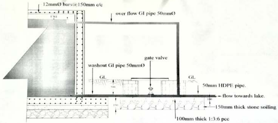
SECTION F-F
