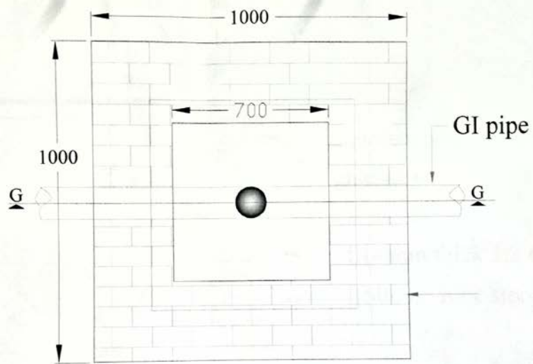
PLAN(valve chamber)
