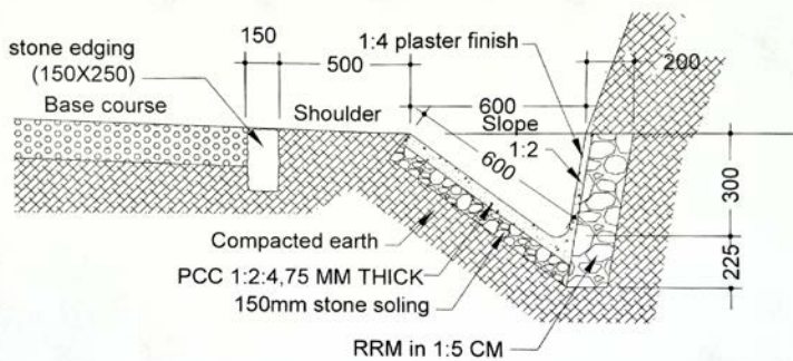
Cross section of Lined V Shaped Drain
